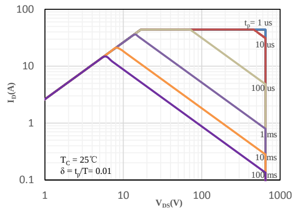
Fig 14 Safe Operation Area (ITO-220AB)
